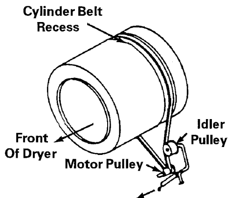
Belt Orientation
