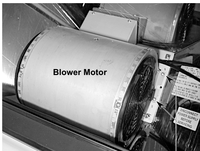
Blower Motor Screws (2 On Each Side)
