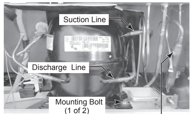
Filter-Drier
