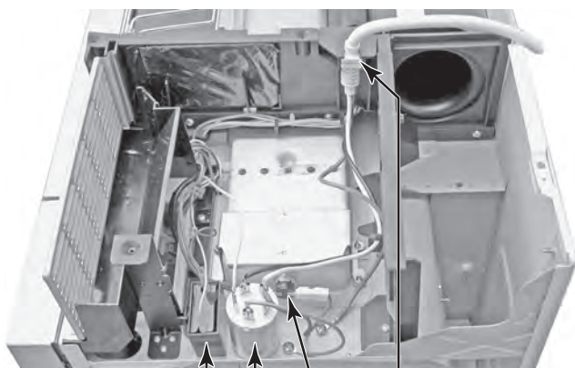
Motor Capacitor AC Line Filter Cavity Thermostat #1 Power Supply Cord
