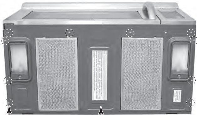
Screw (1 of 10) Bottom Cover Assembly
