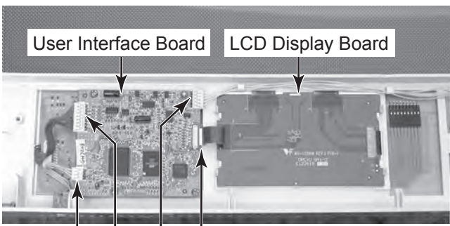
4 Board Connectors
