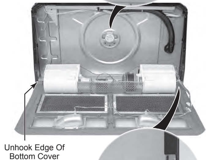
Power Connector
