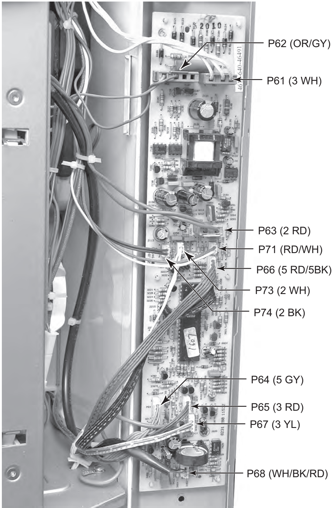
Relay Control Board W/Connectors & Wire Color Callouts
