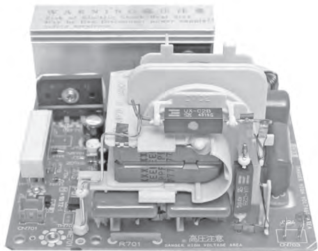
Inverter Board
