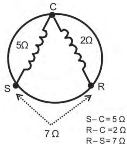
Resistance Checking
