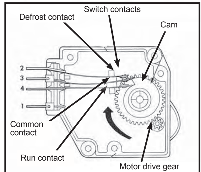
Internal components
