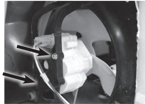
Disconnect wire harness and remove 2 screws securing the motor to the bracket
