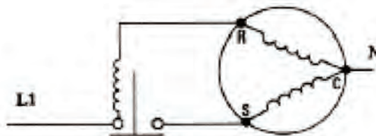
Split phase motor design
