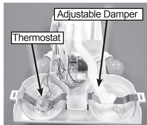
5. Remove housing assembly.
