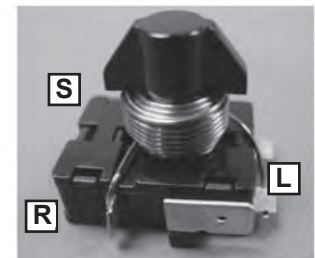
Relay coil wired between L and R
