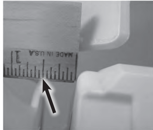
Notate the position of the fan blade on the motor shaft
