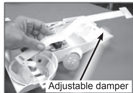
Electro-mechanical thermostat
