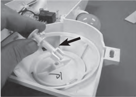
1. Remove shaft.
