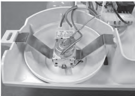
4. Release tab.
