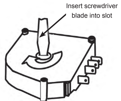
Initiating defrost
