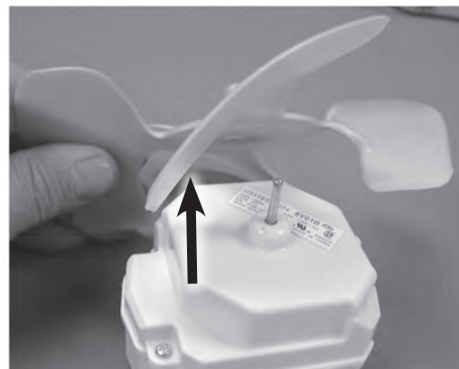
Blade slides off the motor shaft
