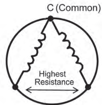
Schematic symbol
