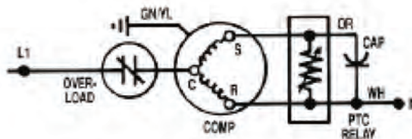
Permanent split capacitor motor design
